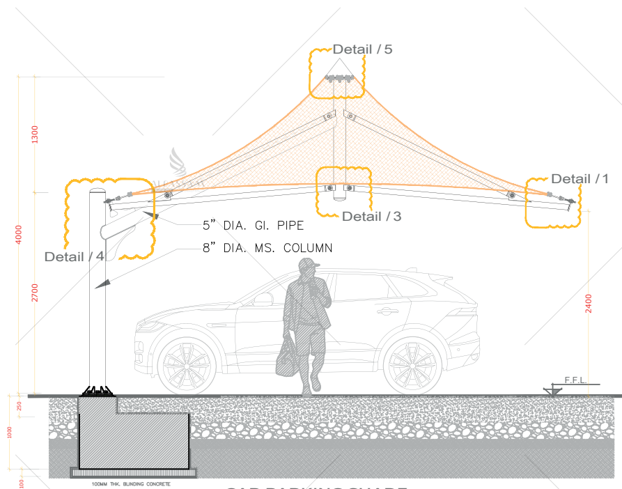
CAR PARKING SHADE SIDE ELEVATION
