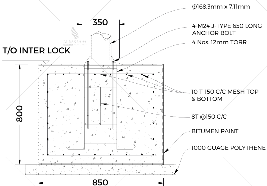
Detail A
