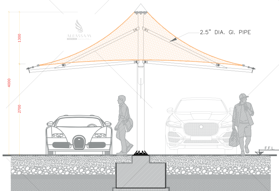
CAR PARKING SHADE FRONT ELEVATION
