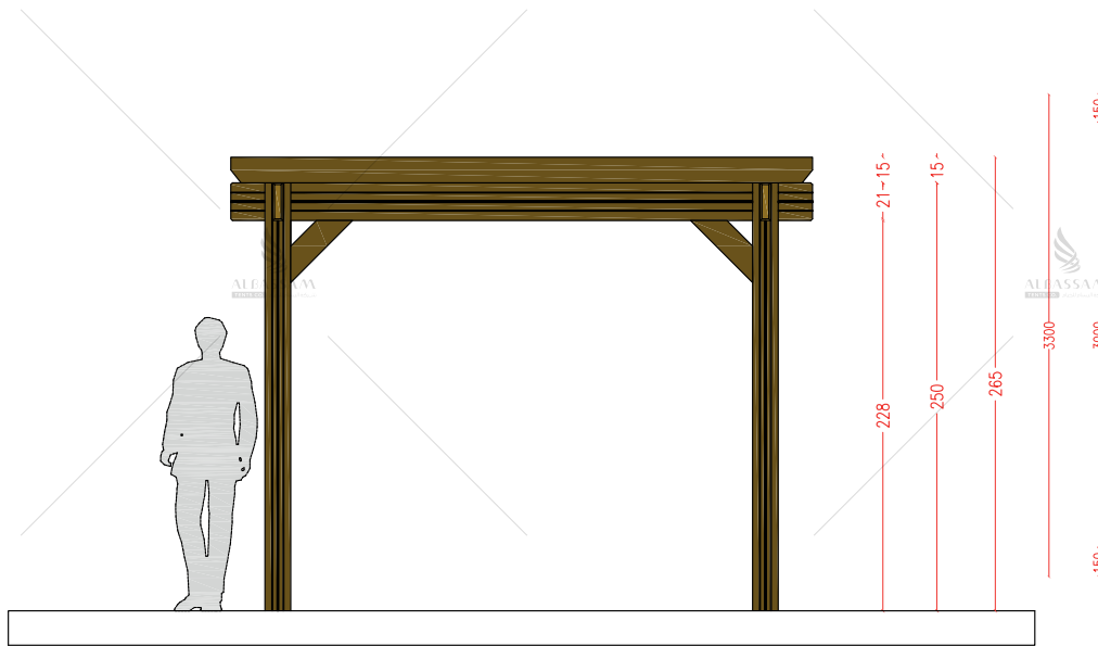
CAR PARKING SHADE SIDE ELEVATION
