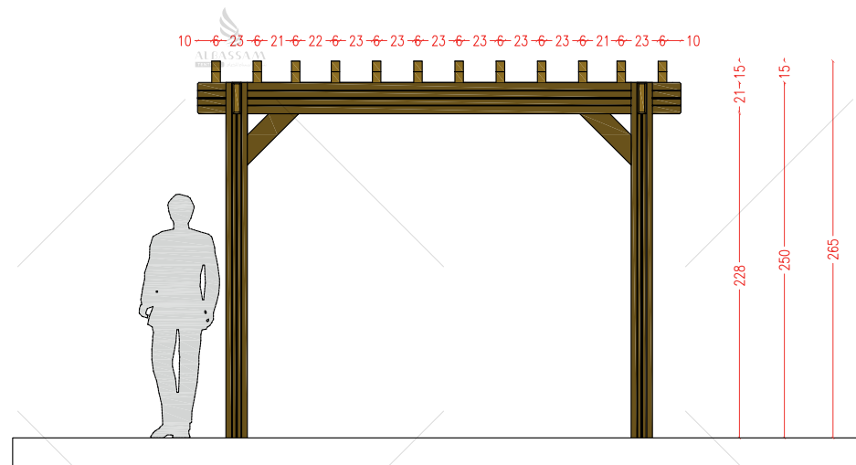
CAR PARKING SHADE FRONT ELEVATION
